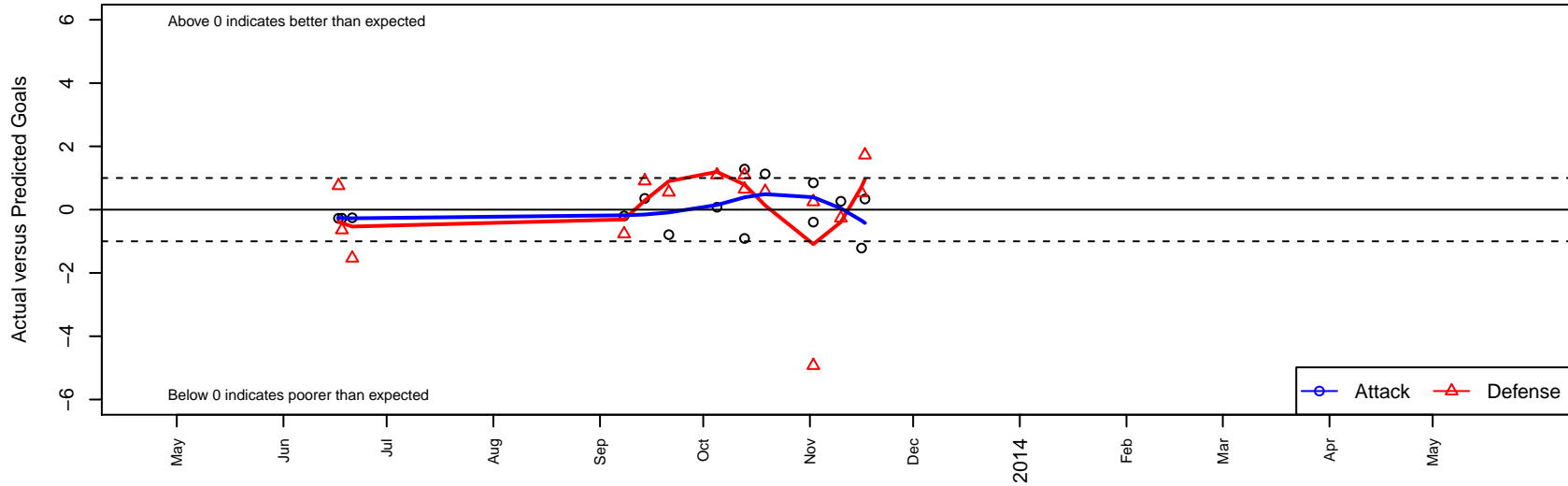
Ceres Earthquakes G00 Dots are actual minus expected GF (blue circles) and GA (red triangles). Blue line is smoothed change in attack strength. Red is smoothed change in defense strength.
